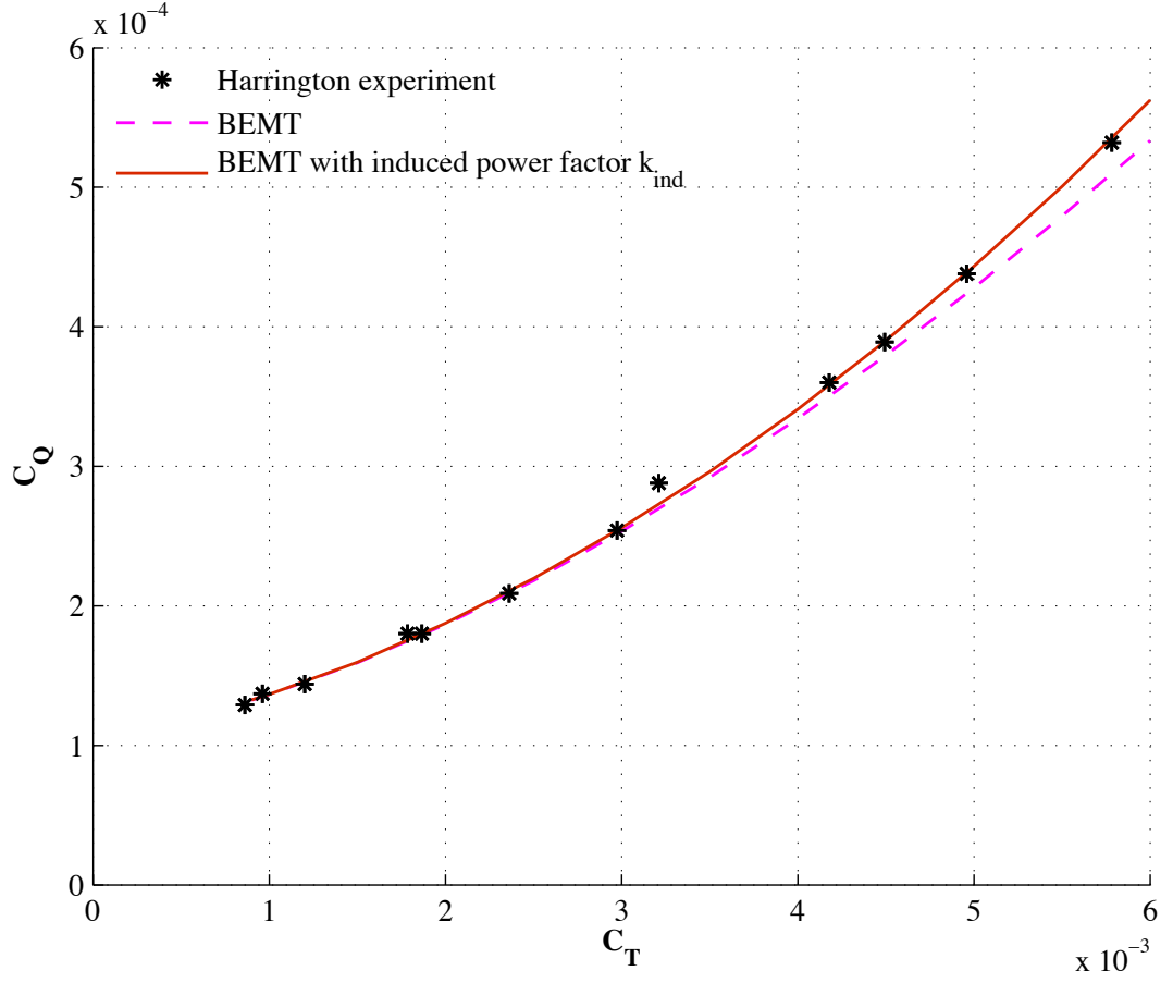
Figure 3.3: OGE validation - BEMT vs experimental results for a rotor with a symmetric NACA airfoil
